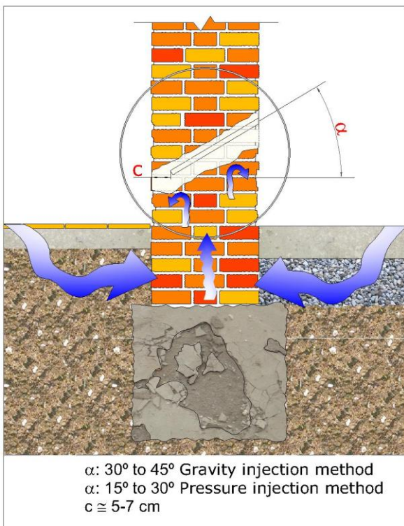
Figure 1. Section wall
